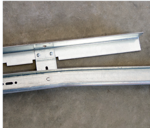
One-piece, curved VL track (for one-man installation)
