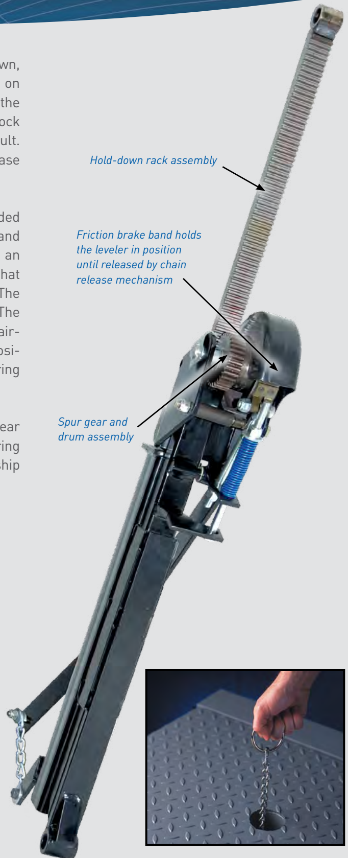
▲ Posi-Trac fingertip leveler release requires only 10 lbs. of lifting force.
